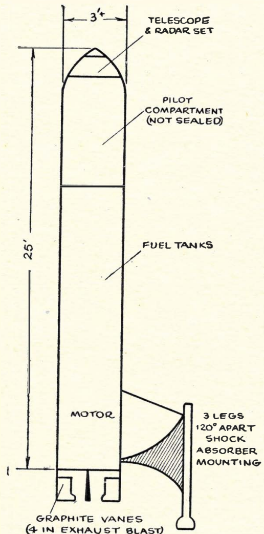
FIGURE 2 One-man space boat, developed from piloted AA rocket
