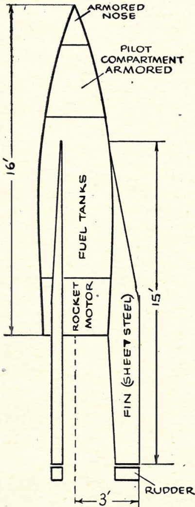
FIGURE 1 Piloted Anti-Aircraft Missile (Lippisch) 3 fins, 120° apart; Booster units between fins, jettisoned at X + 12 seconds
